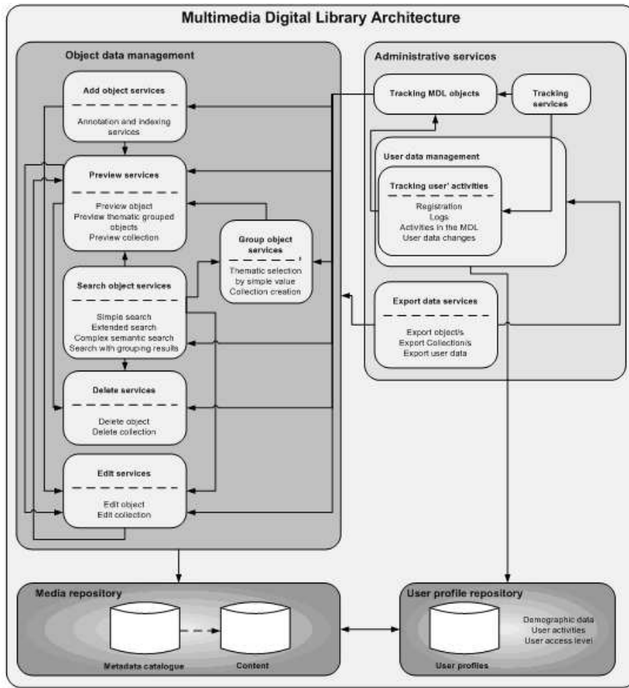
Fig. 1. BIDL Architecture
