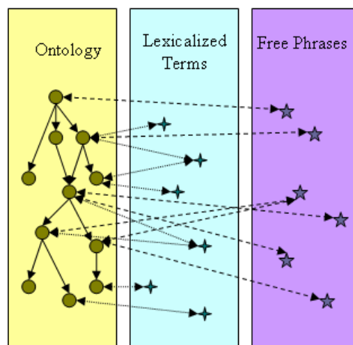
Fig 1. Ontology-to-Lexicon Relation.
