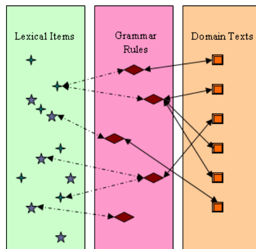
Fig 2. Lexicon-to-Text Relation.
